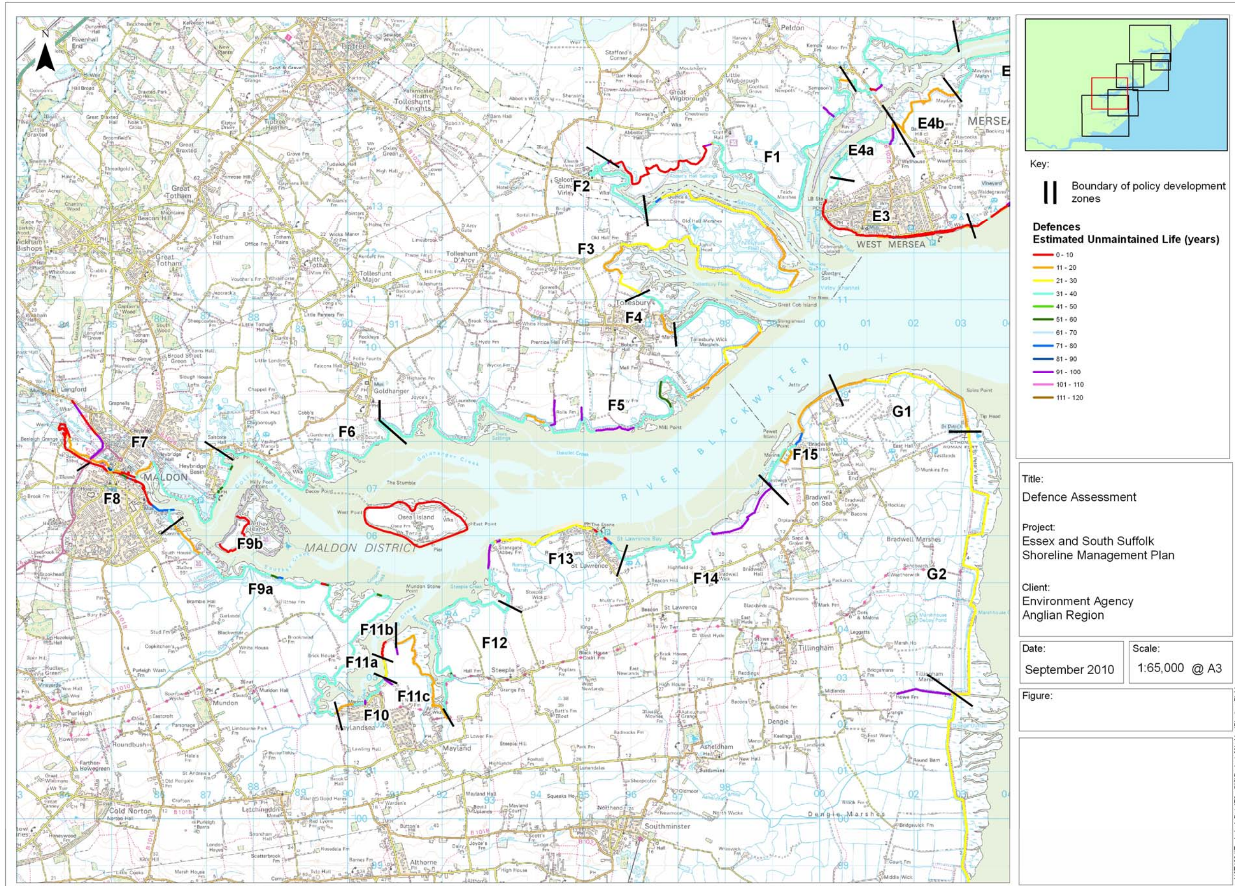
Figure 3-8 Estimated Unmaintained Life of Defences in the Blackwater Estuary
