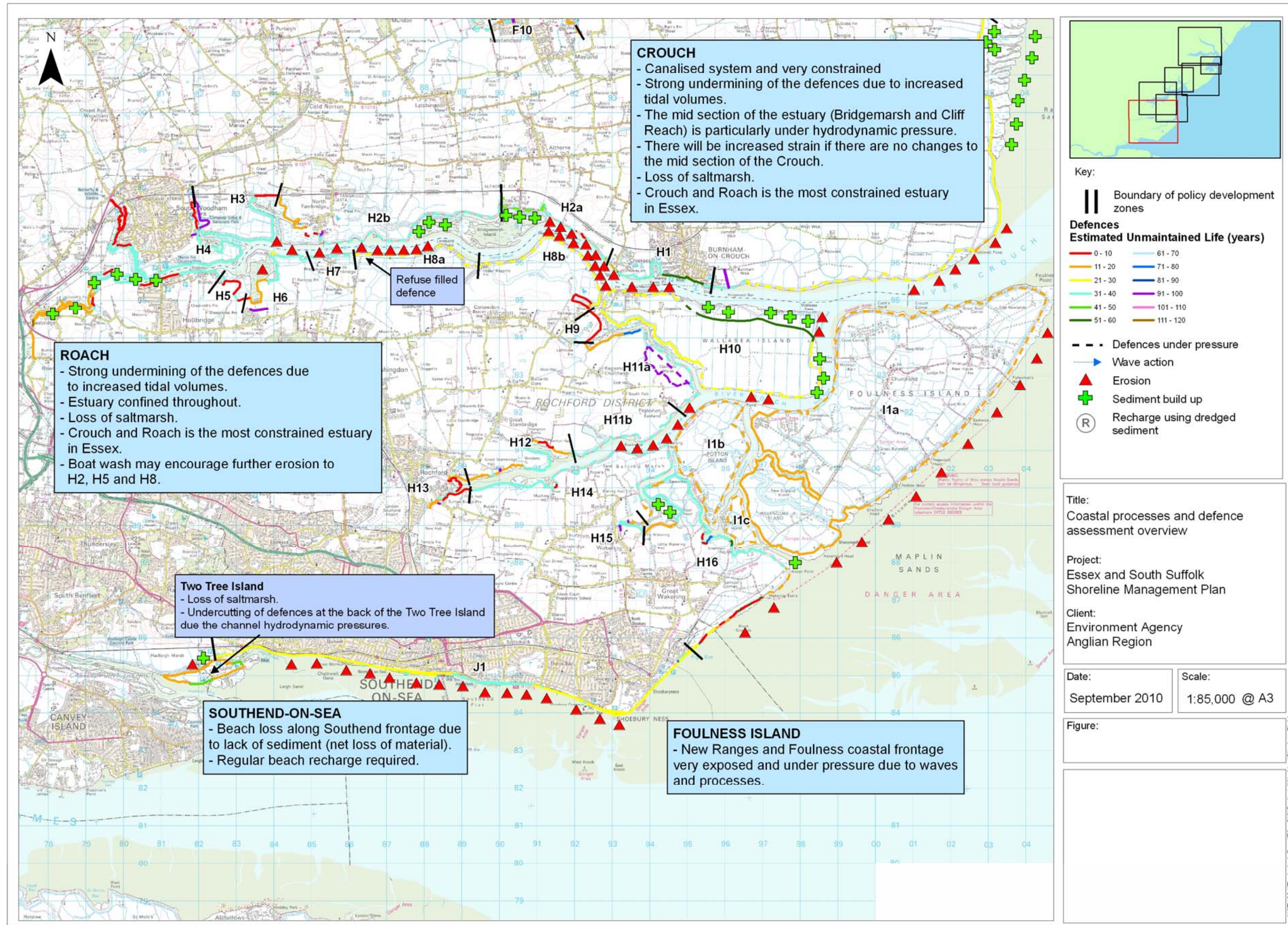
Figure 4-7 Coastal processes and defence assessment overview - Crouch and Roach, Foulness, Potton, Rushley and Southend
